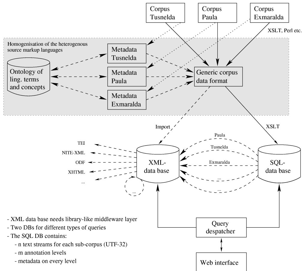
Figure 6: Architecture
